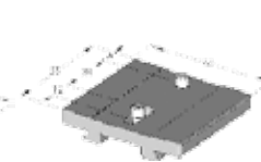
802230 cameraplate 55mm 2x 1/4", d=28-40
